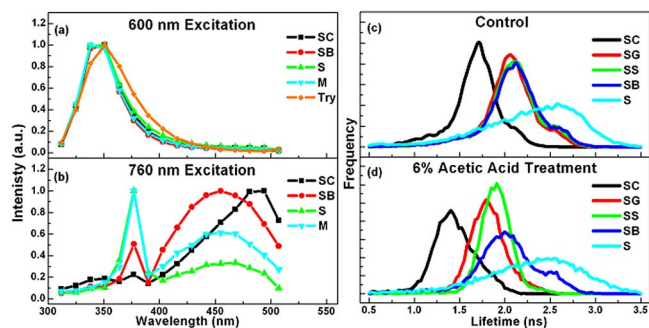
Fig. 2. (Color online) Representative TPEF spectra and lifetime histograms. (a) TPEF spectra excited at 600 nm from SC, SB, S, M, and tryptophan solution (Try); (b) corresponding spectra excited at 760 nm; (c) histograms of tryptophan fluorescence lifetime from SC, SG, SS, SB, and S layers without AA treatment; (d) corresponding histograms with 6% AA treatment.
